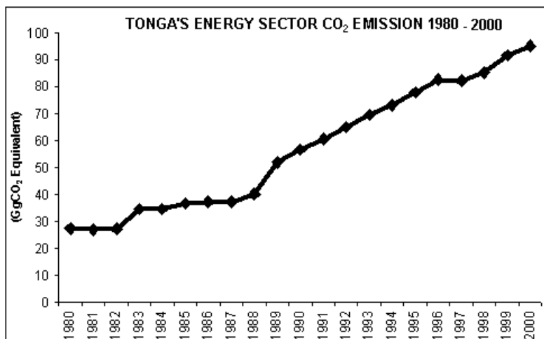
Figure 3: Tonga's Energy Sector CO 2 Emission 1980-2000
